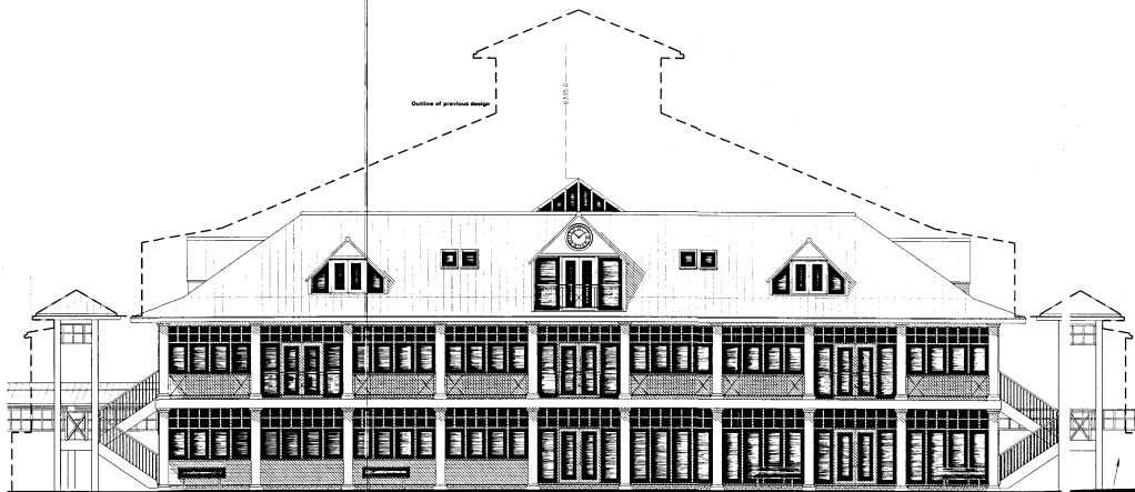
Rear Elevation
